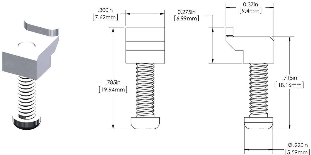
Figure 31: Cleat assembly
