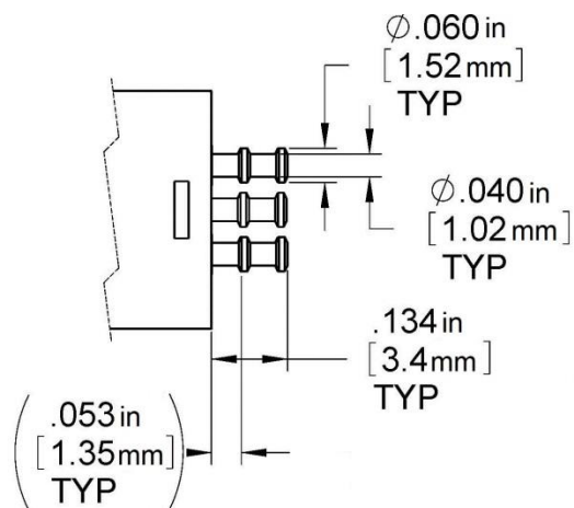
Figure 6: Solder termination
