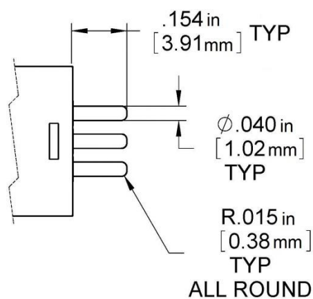
Figure 7: PC termination
